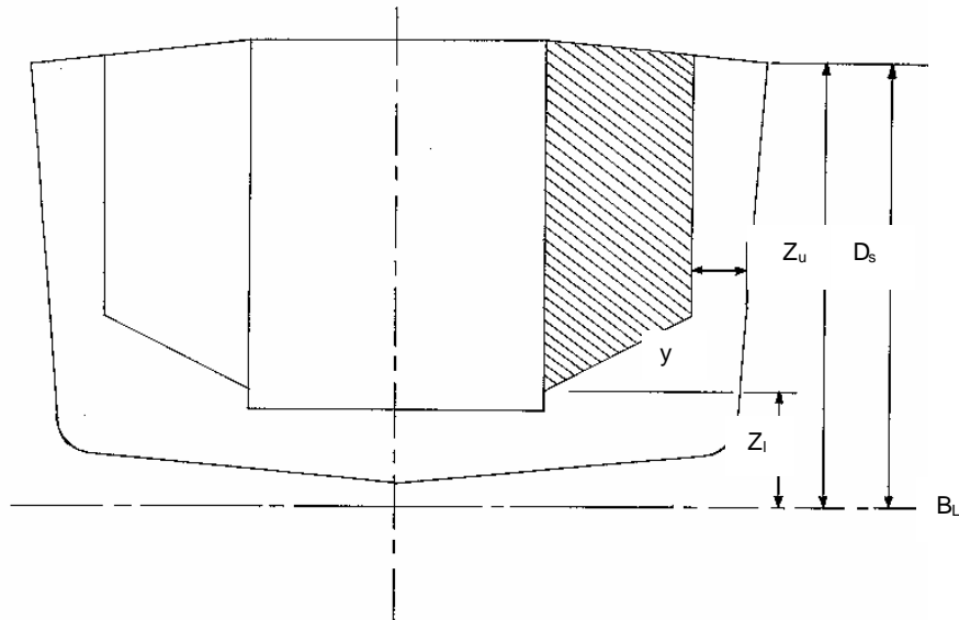
Figure 18 – Z_u , Z_i and y for outer cargo tank (Section looking forward)
