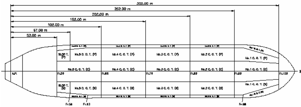
Figure 27 - Tank Arrangement
