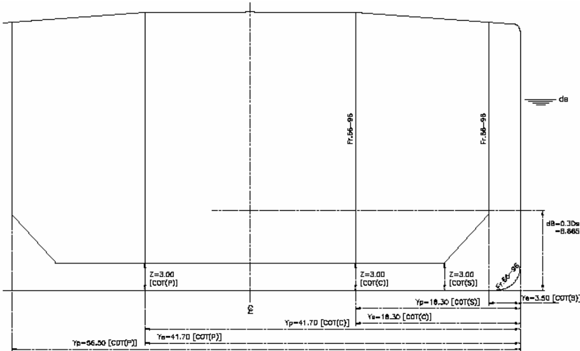
Figure 32 - Bottom Damage (Nos. 2,3,4 COT (Fr.66-Fr.96))
