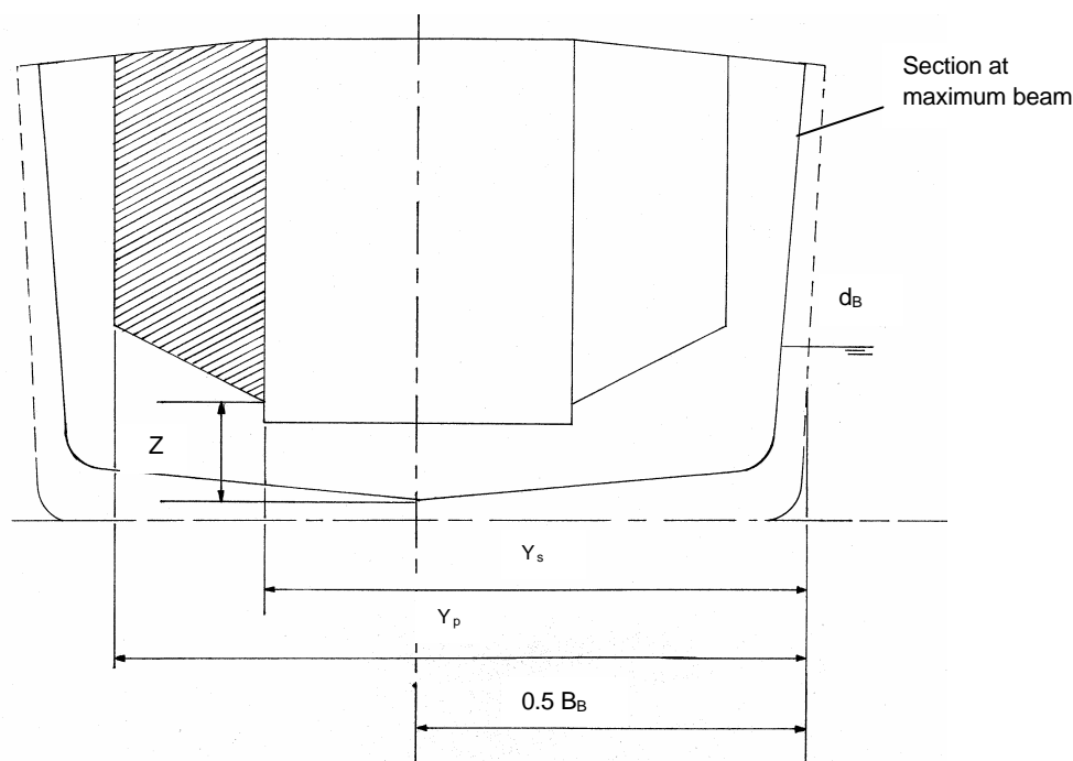
Figure 23 – Y_s , Y_p and z for port cargo tank (Section looking forward)
