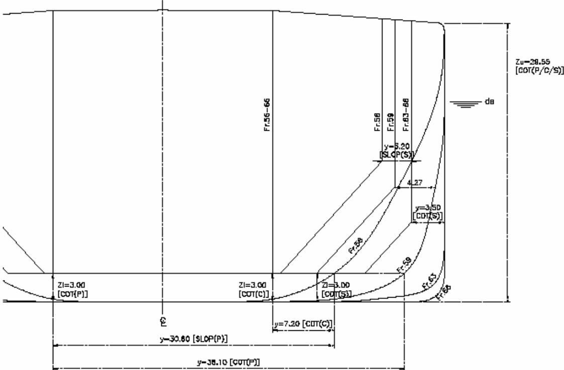
Figure 30 - Side Damage (No.5 COT & SLOP (Fr. 56-Fr.66))
