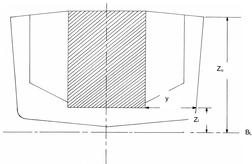
Figure 19 – Z_u , Z_i and y for centre cargo tank (Section looking forward)
