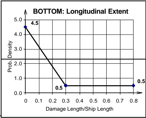
Figure 8 - Bottom Damage: Longitudinal Extent
