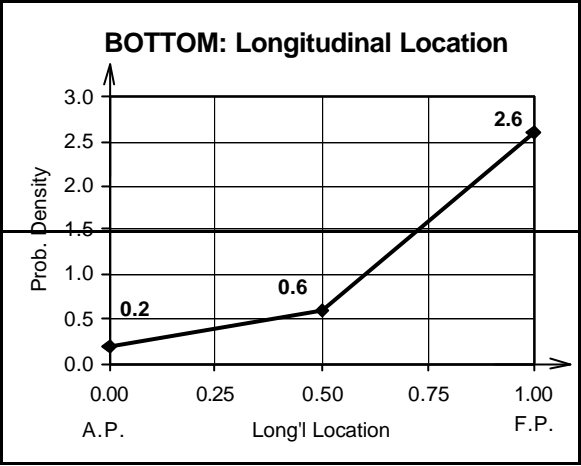
Figure 7 - Bottom Damage: Longitudinal Location
