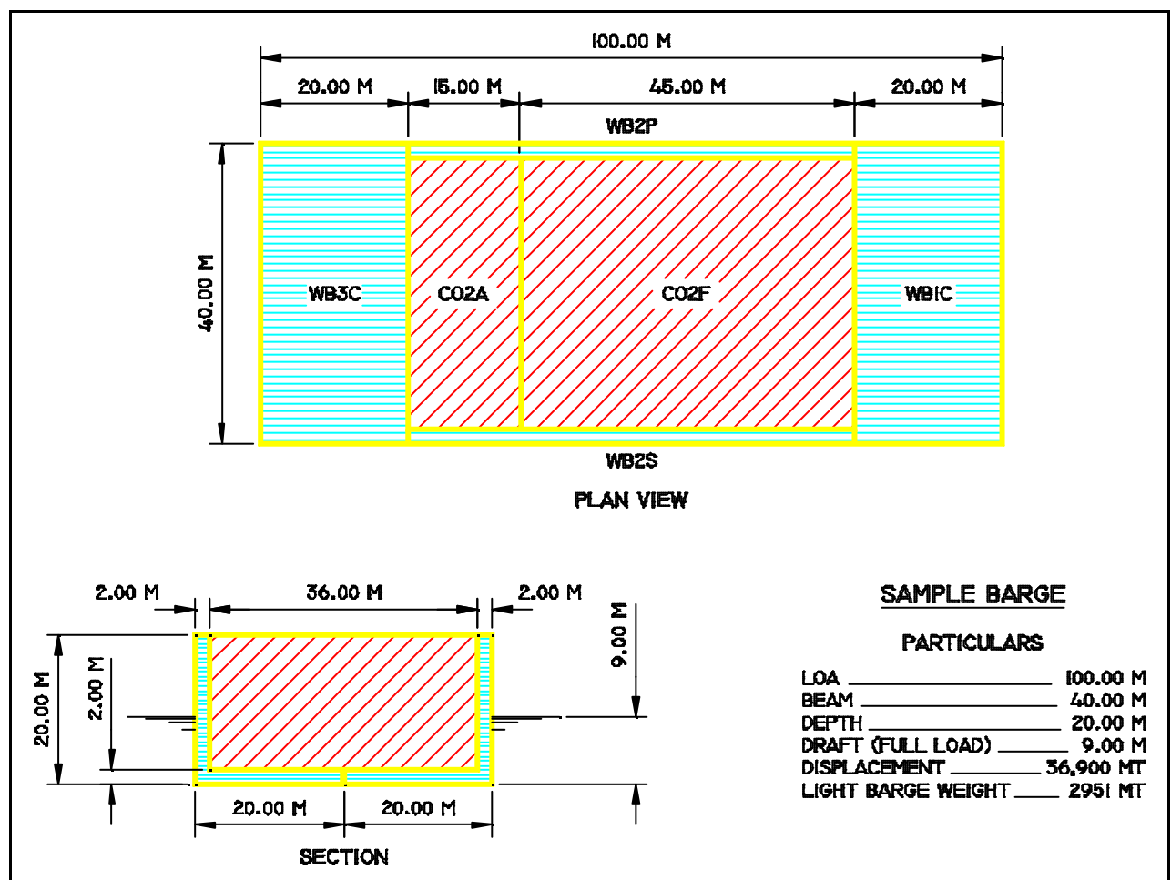
Figure 26 – Barge Arrangement
